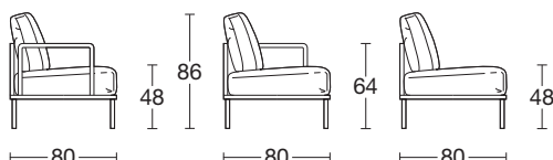
VISTA LATERALE SIDE VIEW
